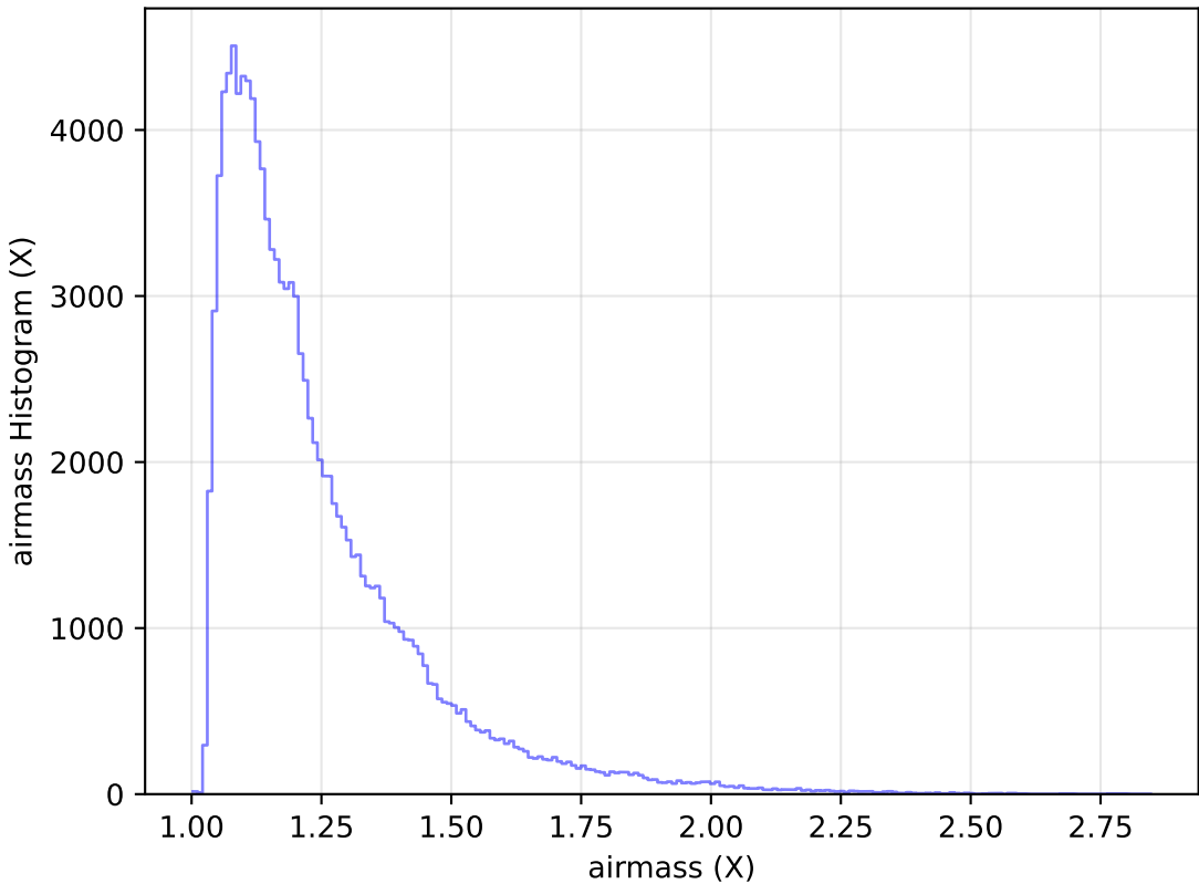
extra_ss_neo3_v3.4_10yrs All sky u band: airmass Histogram
