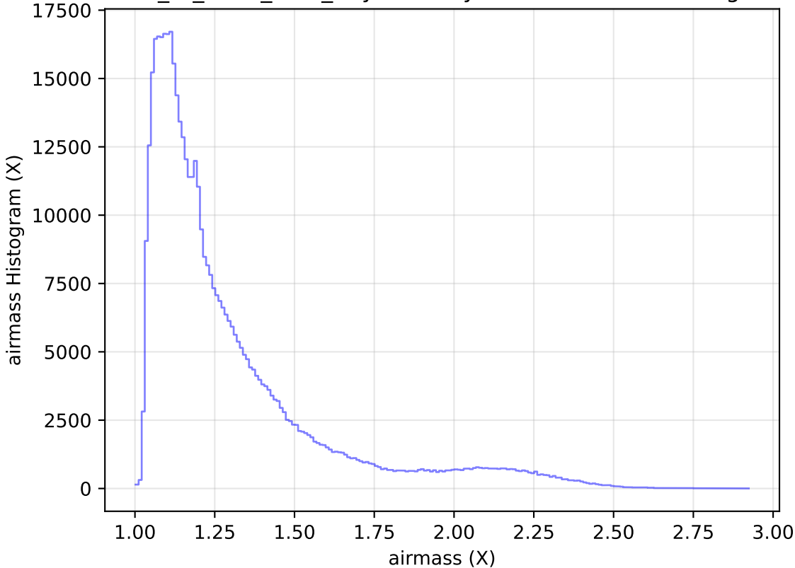
extra_ss_neo3_v3.4_10yrs All sky r band: airmass Histogram
