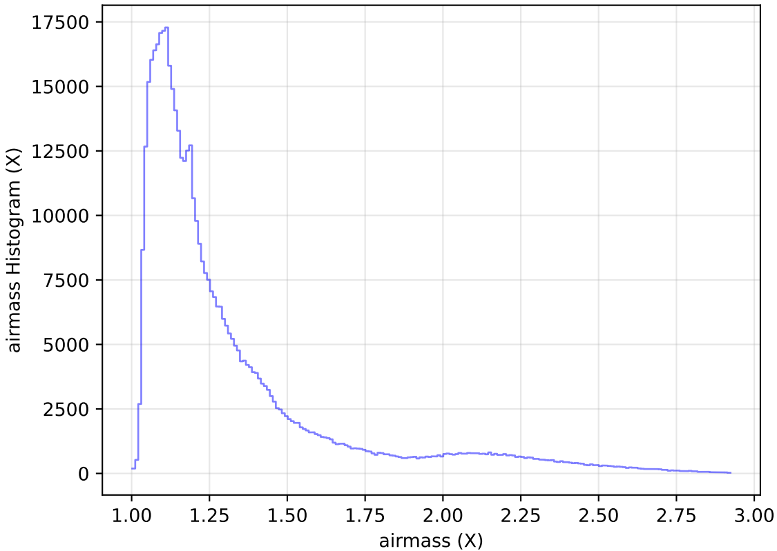
extra_ss_neo3_v3.4_10yrs All sky i band: airmass Histogram
