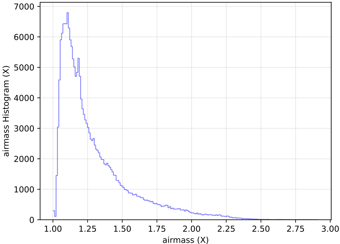
extra_ss_neo3_v3.4_10yrs All sky g band: airmass Histogram
