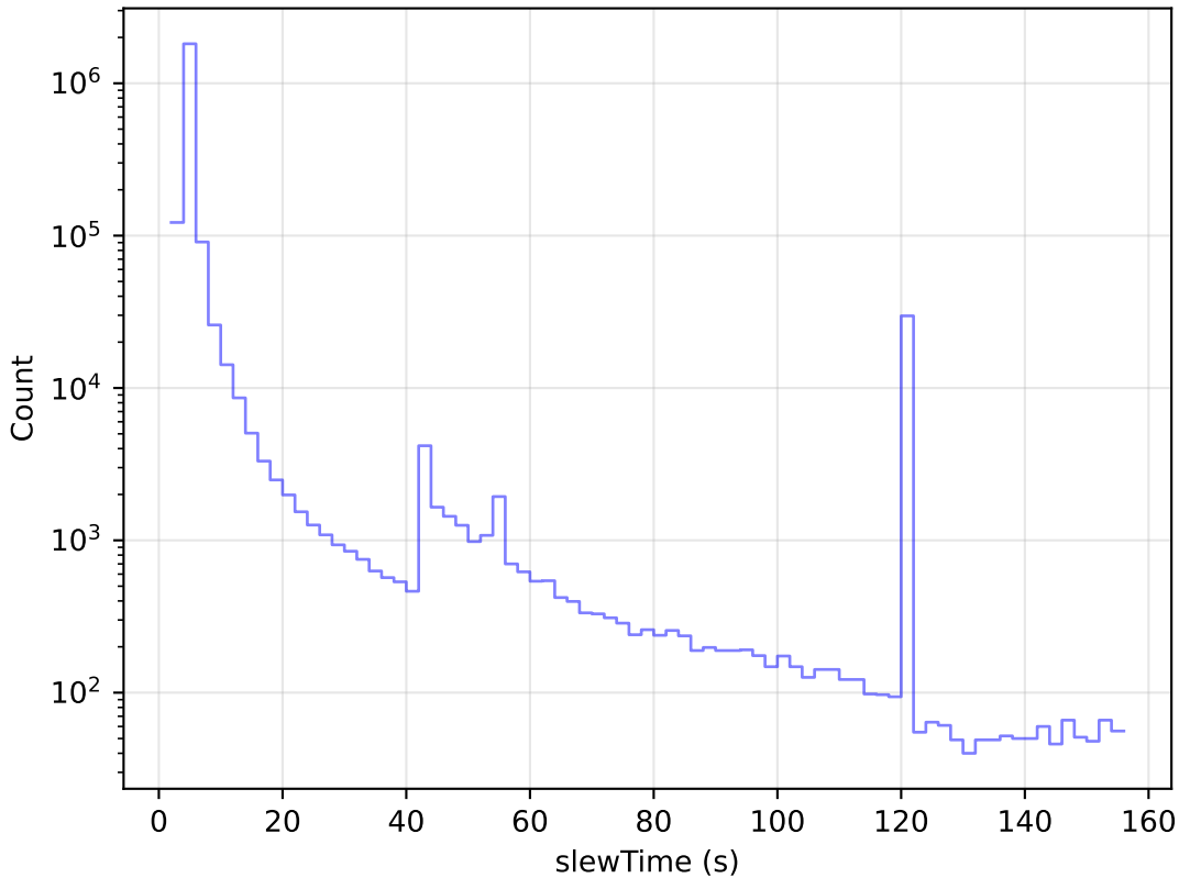
extra_ss_neo3_v3.4_10yrs All visits: Slew Time Histogram
