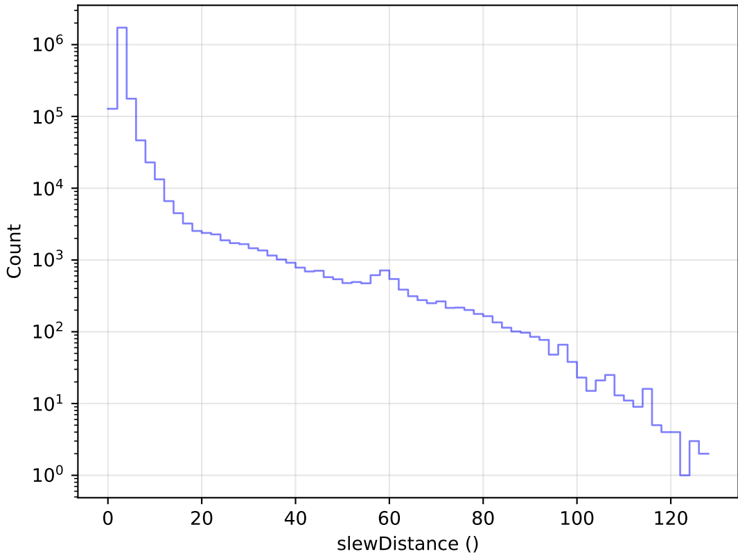
extra_ss_neo3_v3.4_10yrs All visits: Slew Distance Histogram
