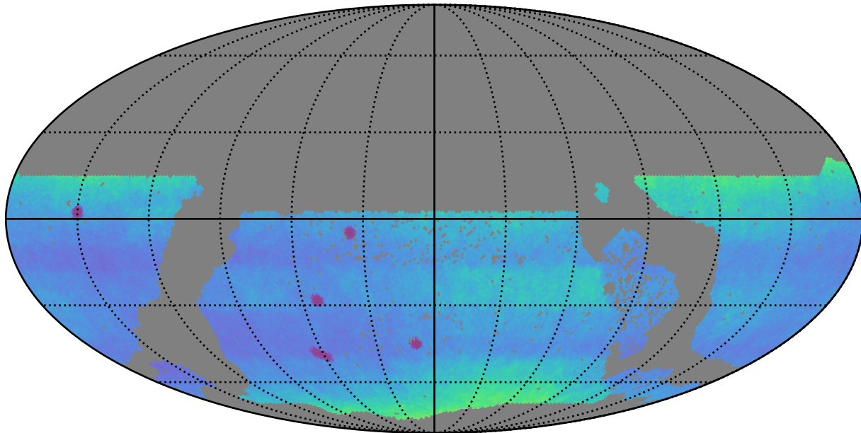
extra_ss_neo3_v3.4_10yrs WFD: Proper Motion Uncert @ 24.0
