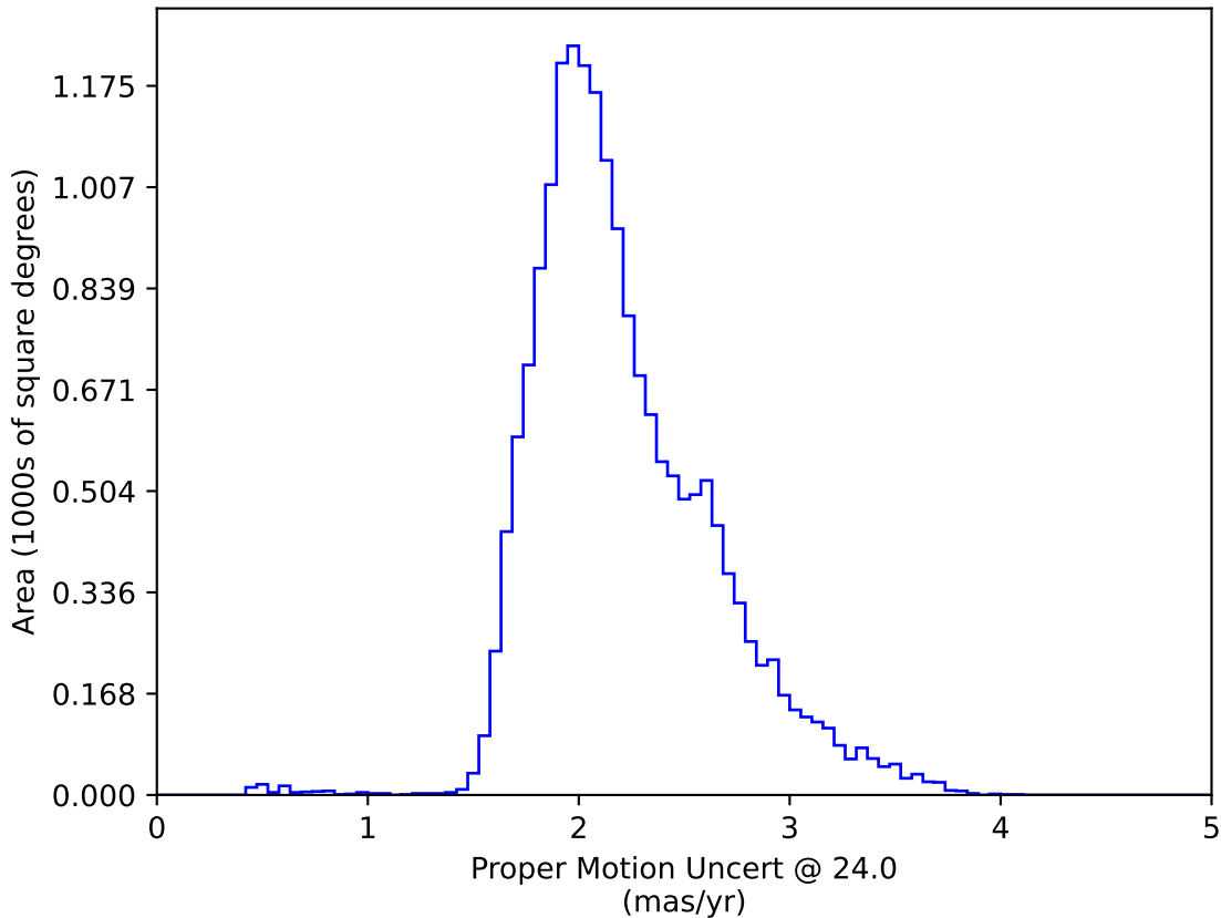
extra_ss_neo3_v3.4_10yrs WFD: Proper Motion Uncert @ 24.0
