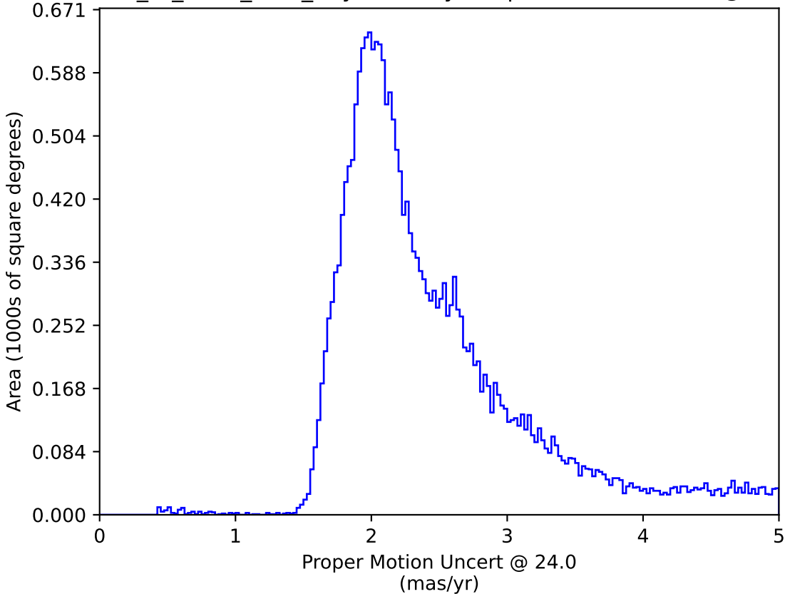
extra_ss_neo3_v3.4_10yrs All sky: Proper Motion Uncert @ 24.0
