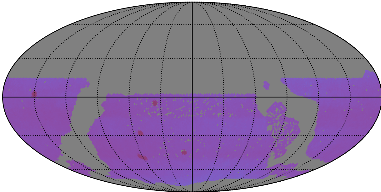
extra_ss_neo3_v3.4_10yrs WFD: Proper Motion Uncert @ 20.5
