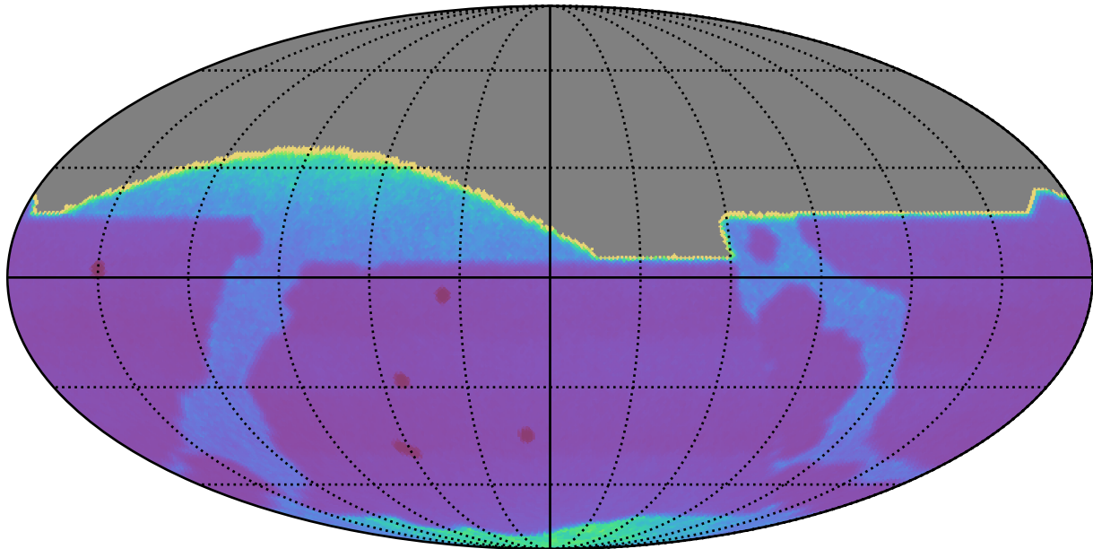
extra_ss_neo3_v3.4_10yrs All sky: Proper Motion Uncert @ 20.5
