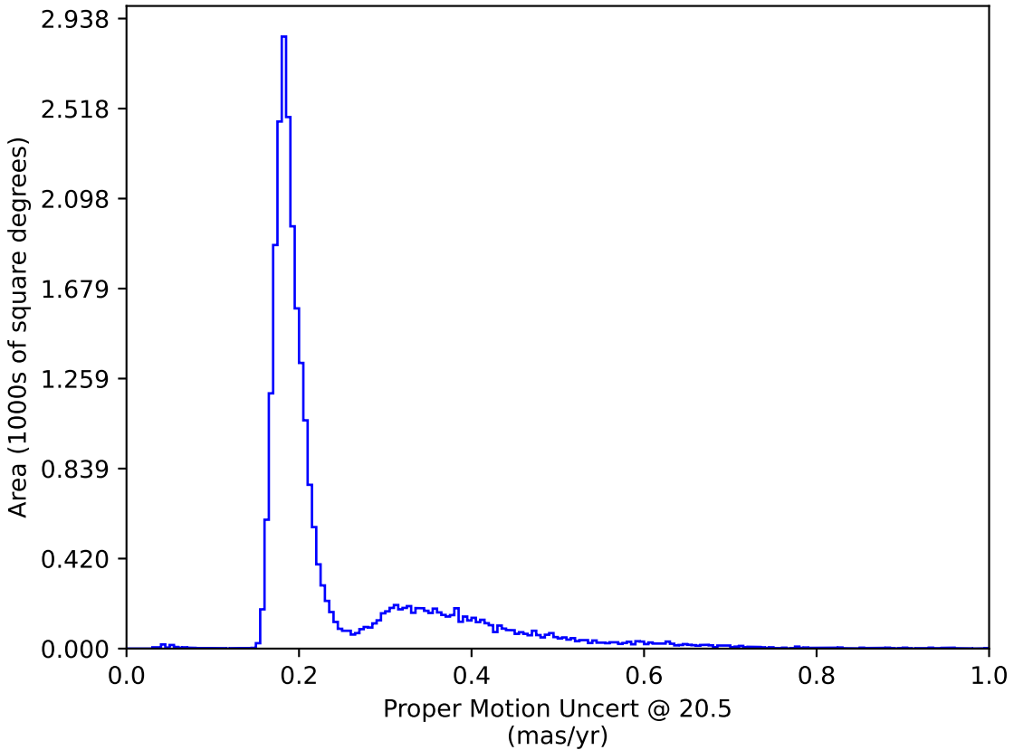
extra_ss_neo3_v3.4_10yrs All sky: Proper Motion Uncert @ 20.5
