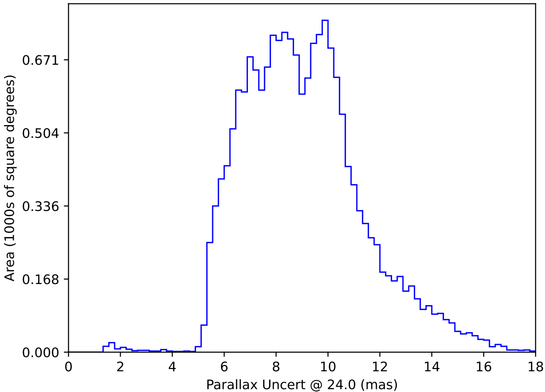
extra_ss_neo3_v3.4_10yrs WFD: Parallax Uncert @ 24.0
