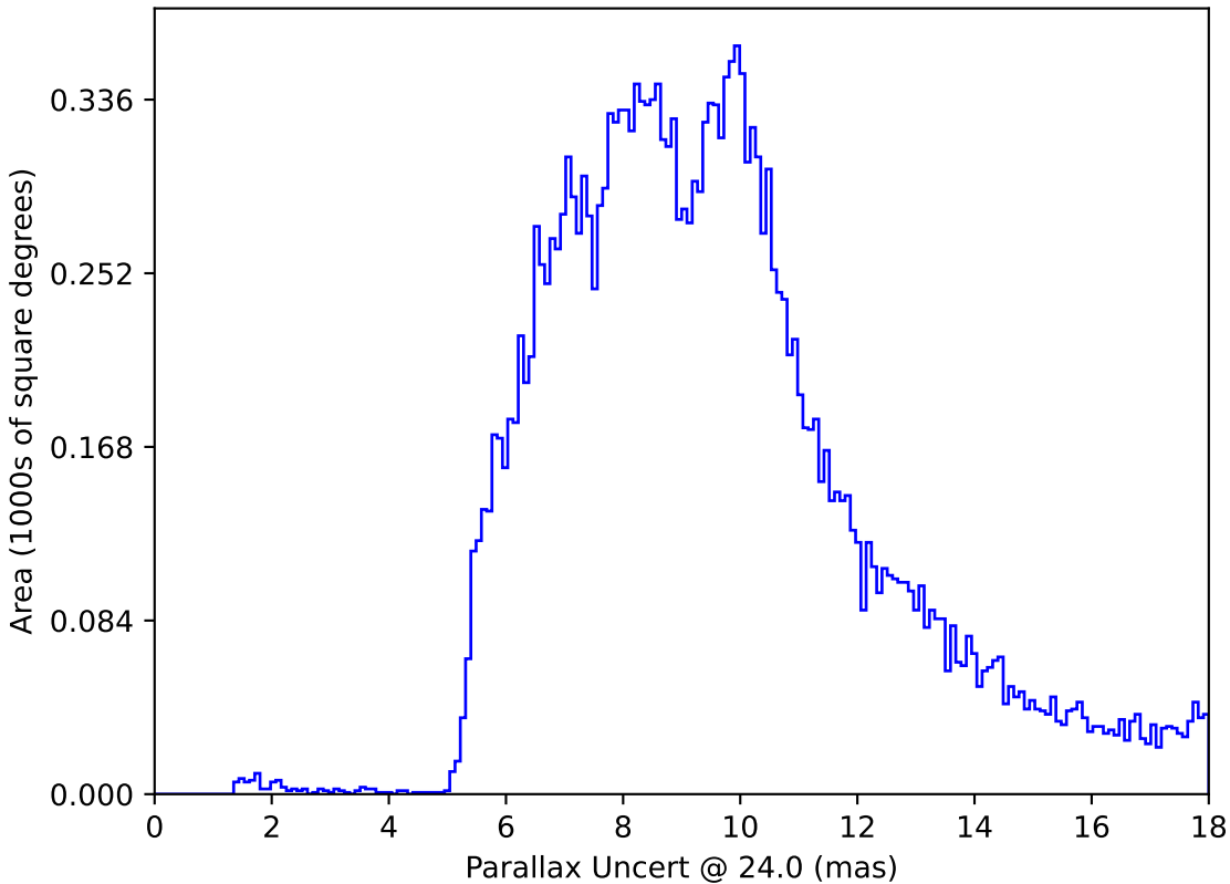
extra_ss_neo3_v3.4_10yrs All sky: Parallax Uncert @ 24.0
