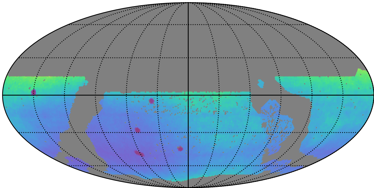
extra_ss_neo3_v3.4_10yrs WFD: Parallax Uncert @ 22.4
