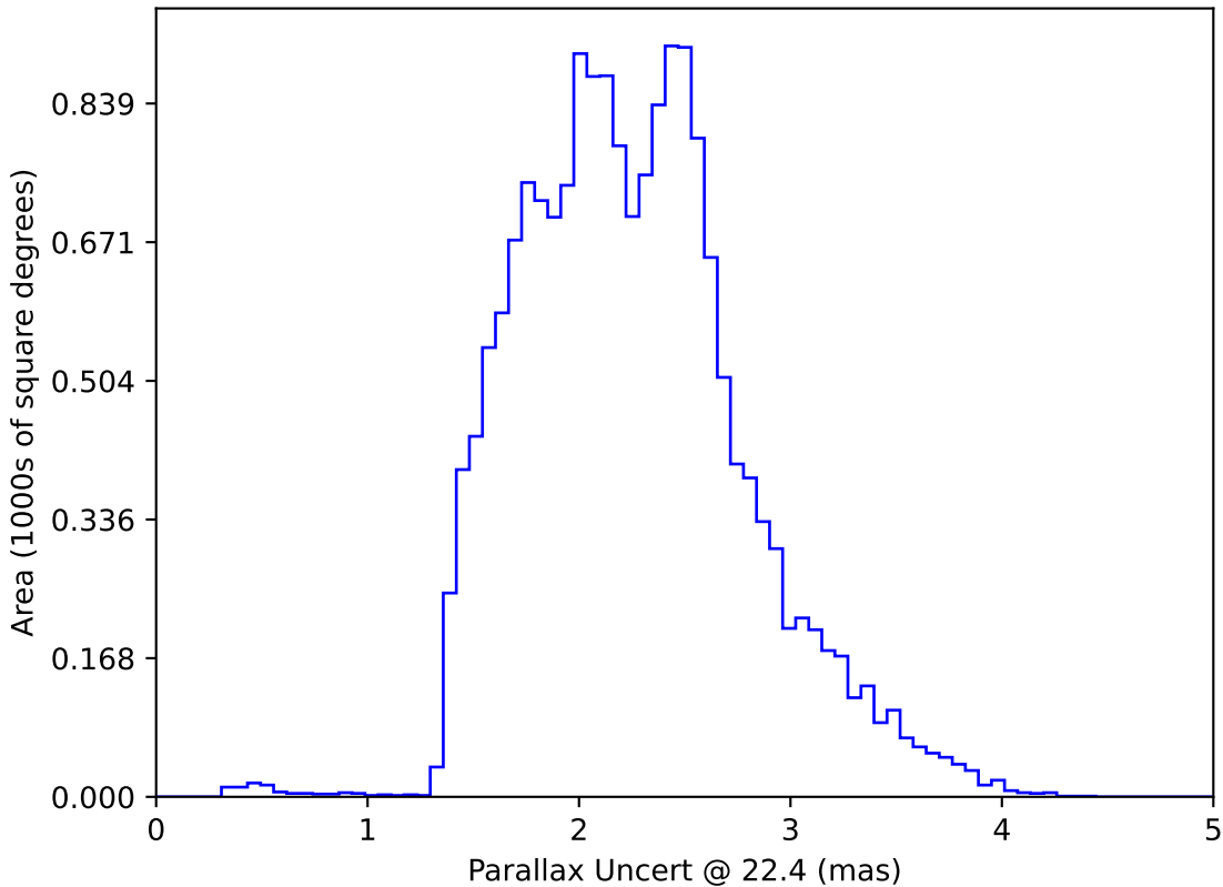
extra_ss_neo3_v3.4_10yrs WFD: Parallax Uncert @ 22.4
