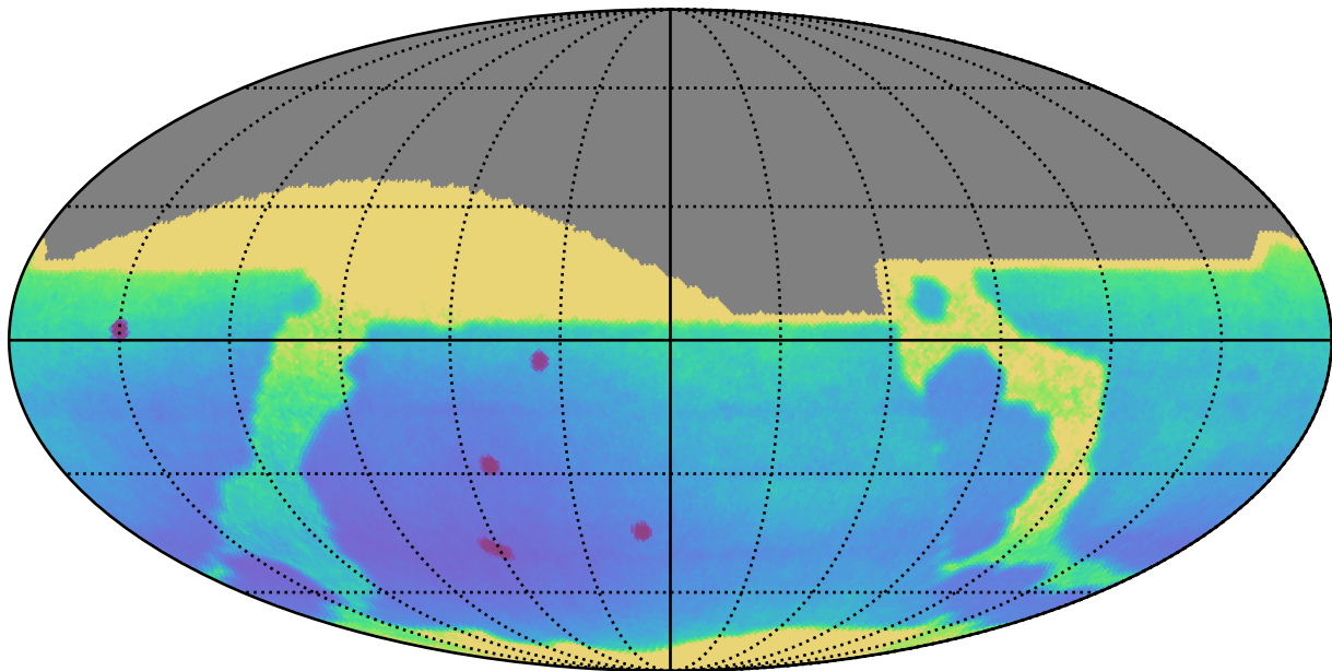
extra_ss_neo3_v3.4_10yrs All sky: Parallax Uncert @ 22.4
