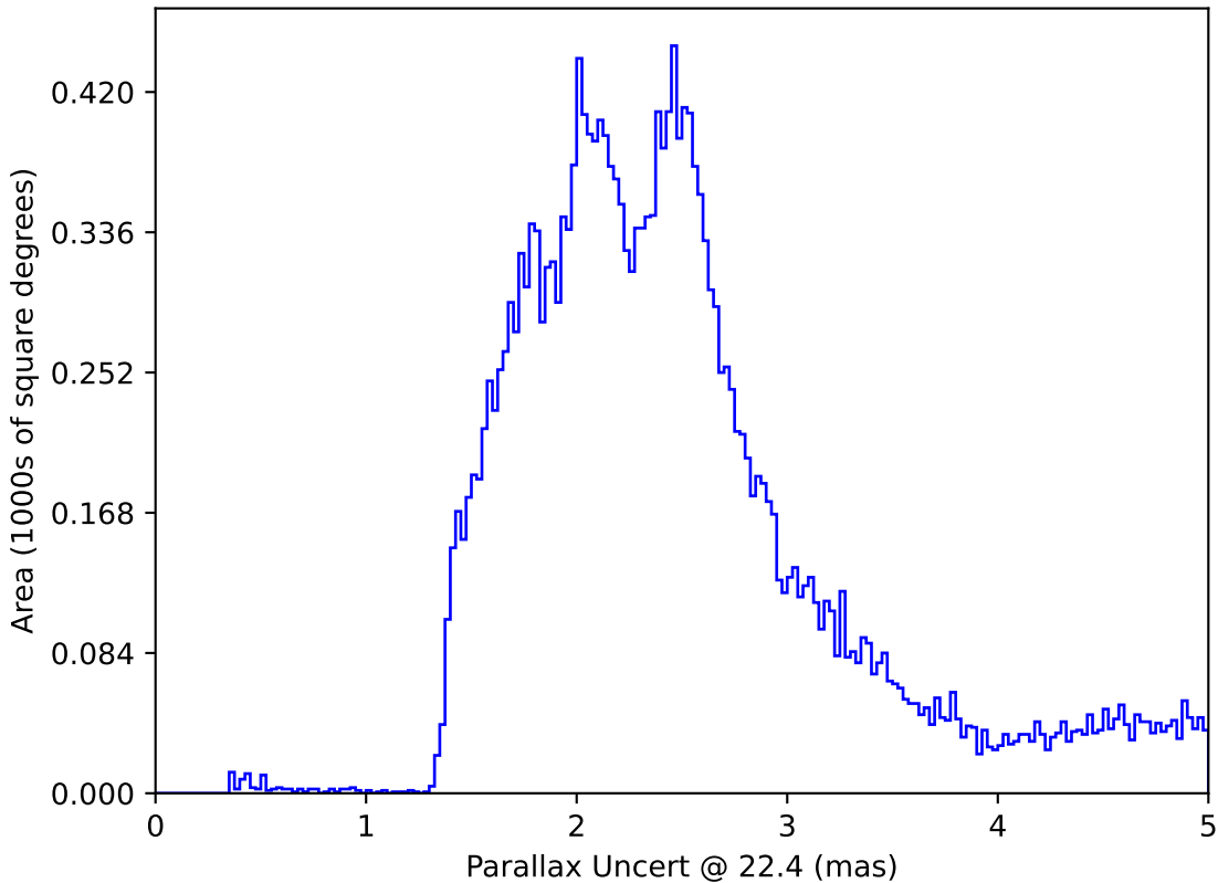
extra_ss_neo3_v3.4_10yrs All sky: Parallax Uncert @ 22.4
