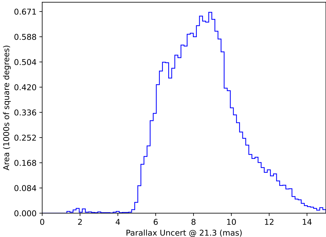
extra_ss_neo3_v3.4_10yrs WFD y band only: Parallax Uncert @ 21.3
