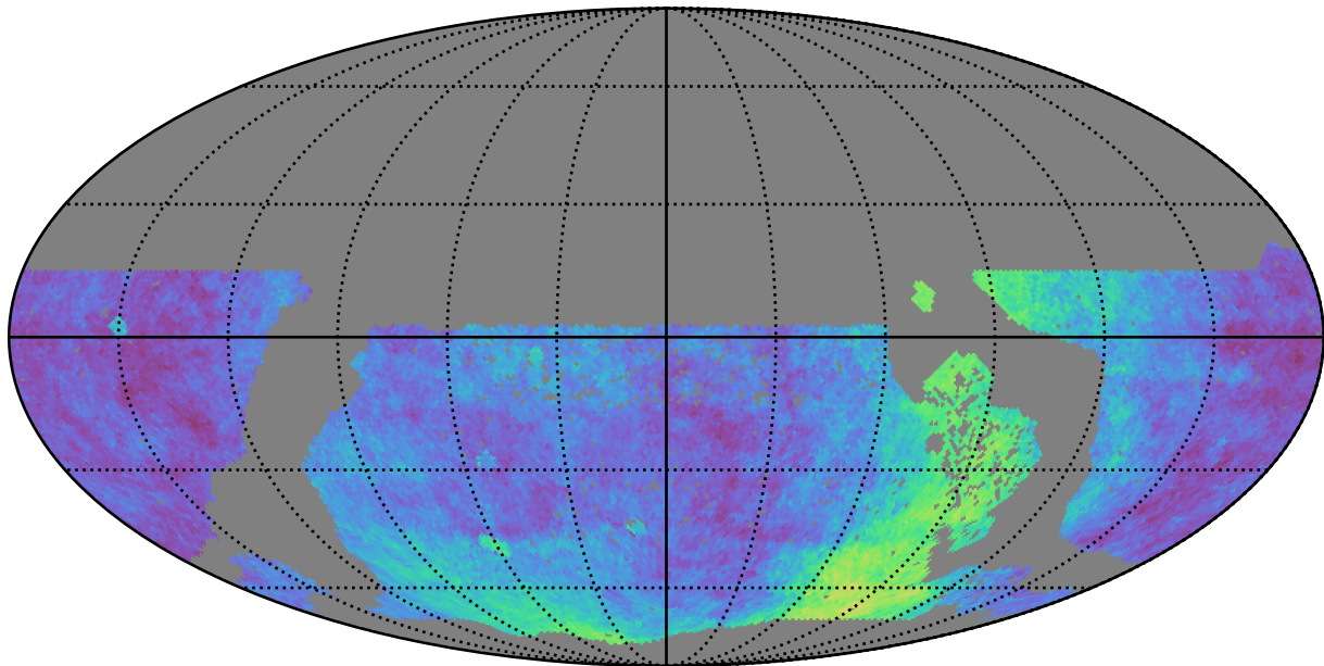
extra_ss_neo3_v3.4_10yrs WFD: Parallax Coverage @ 24.0
