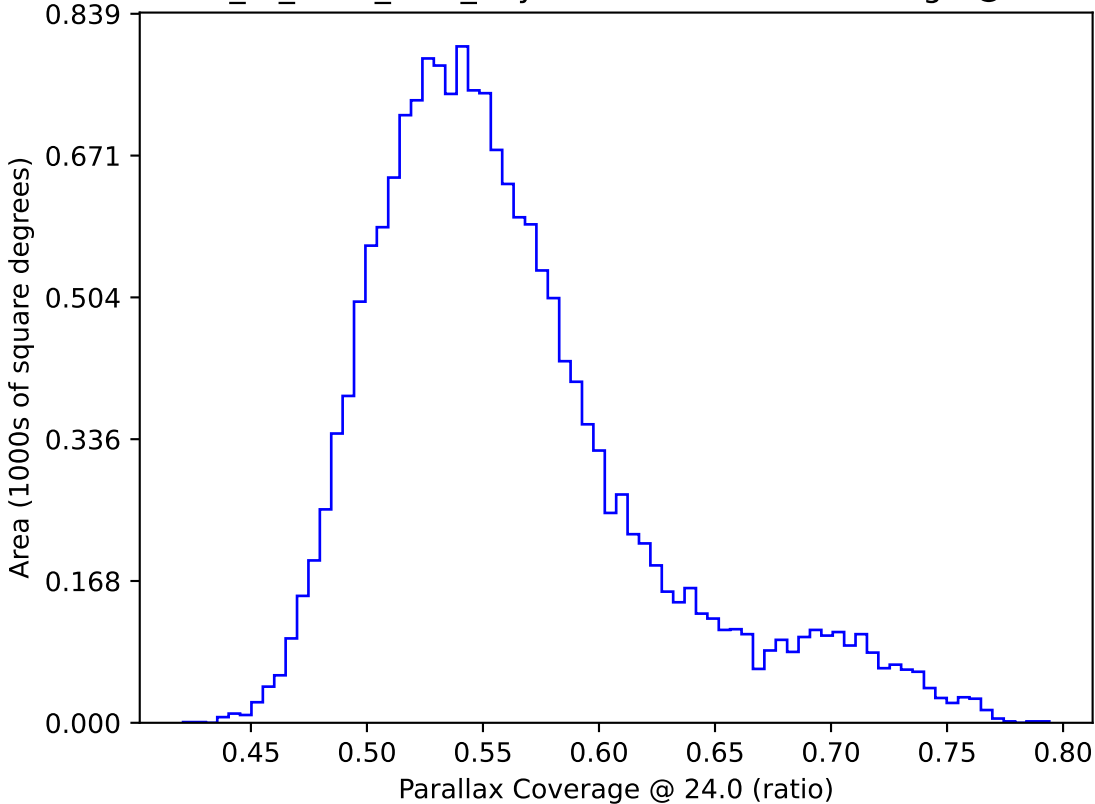
extra_ss_neo3_v3.4_10yrs WFD: Parallax Coverage @ 24.0
