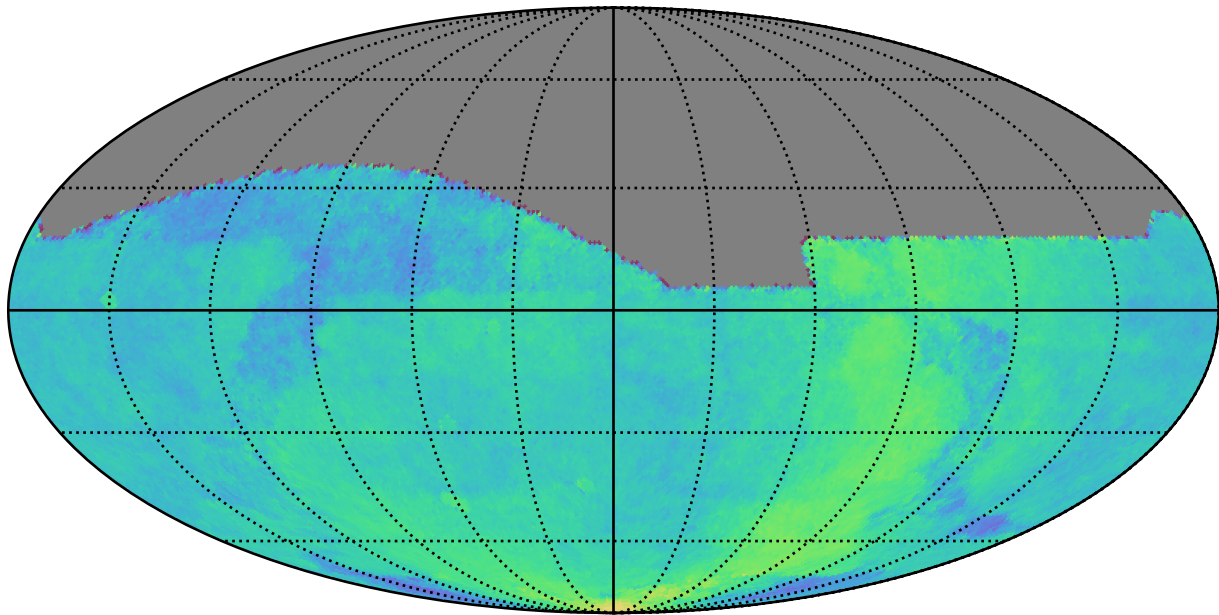
extra_ss_neo3_v3.4_10yrs All sky: Parallax Coverage @ 24.0
