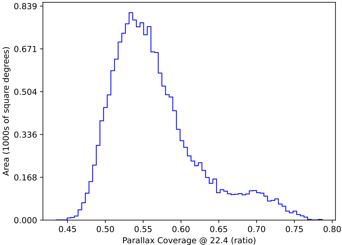
extra_ss_neo3_v3.4_10yrs WFD: Parallax Coverage @ 22.4
