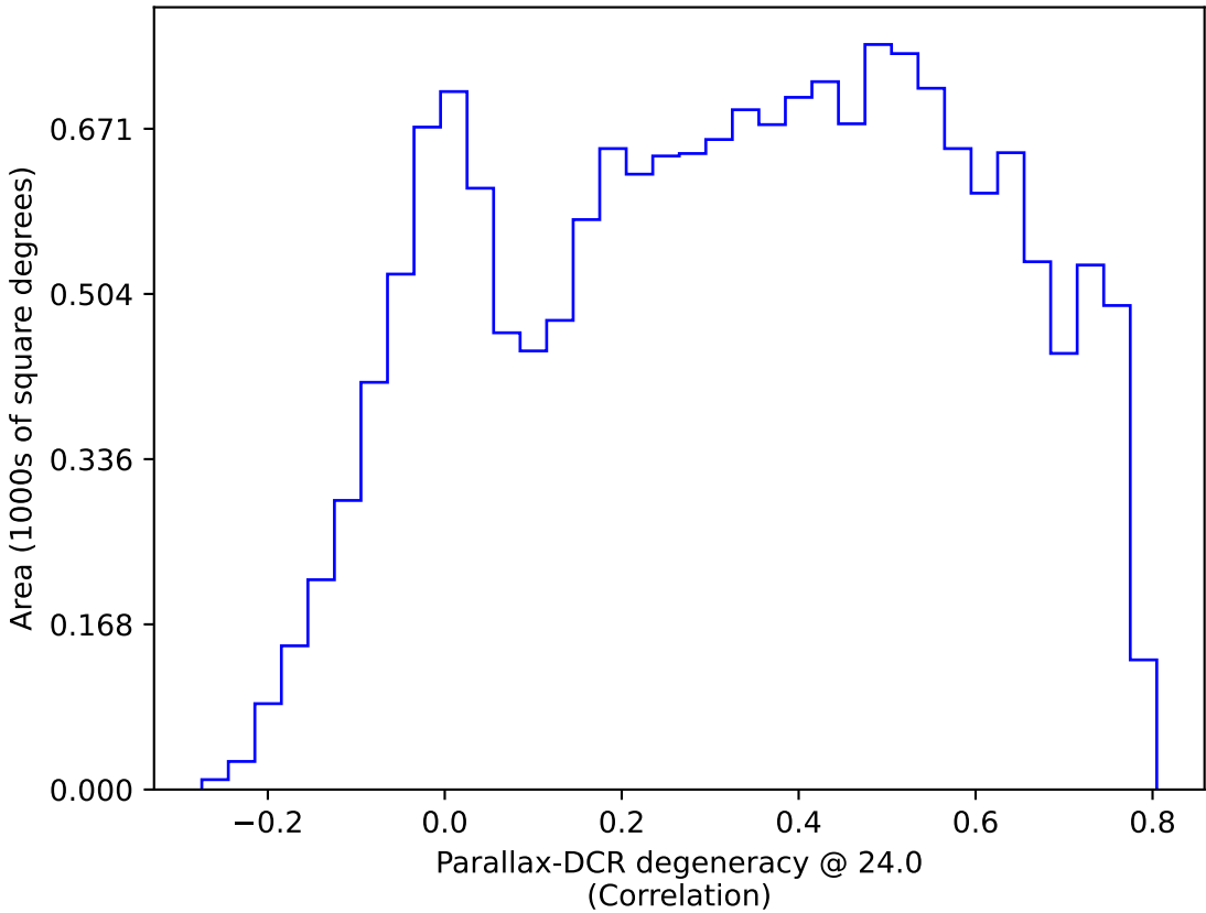
extra_ss_neo3_v3.4_10yrs WFD: Parallax-DCR degeneracy @ 24.0
