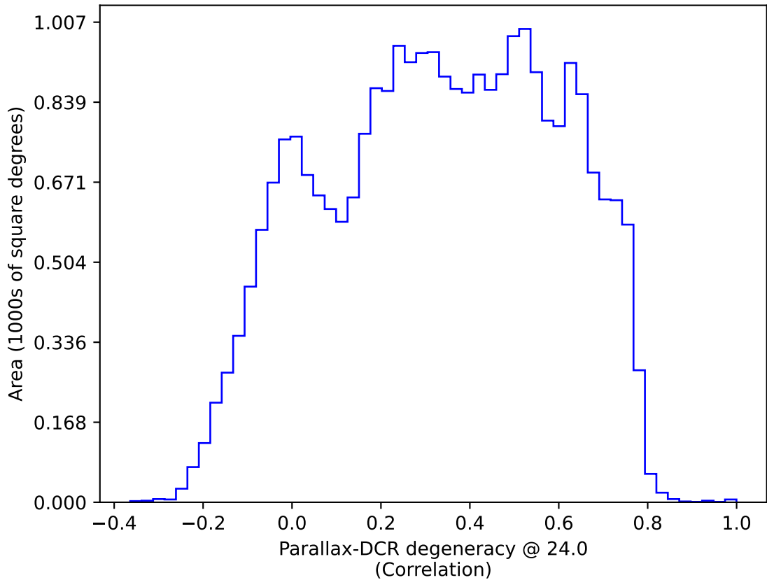
extra_ss_neo3_v3.4_10yrs All sky: Parallax-DCR degeneracy @ 24.0
