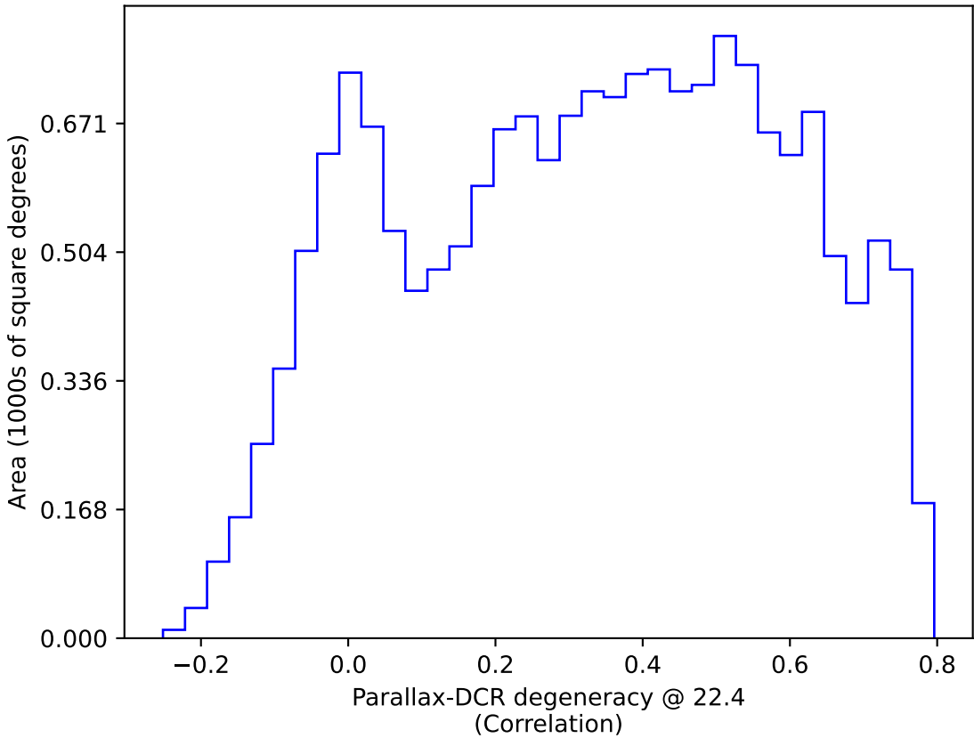
extra_ss_neo3_v3.4_10yrs WFD: Parallax-DCR degeneracy @ 22.4
