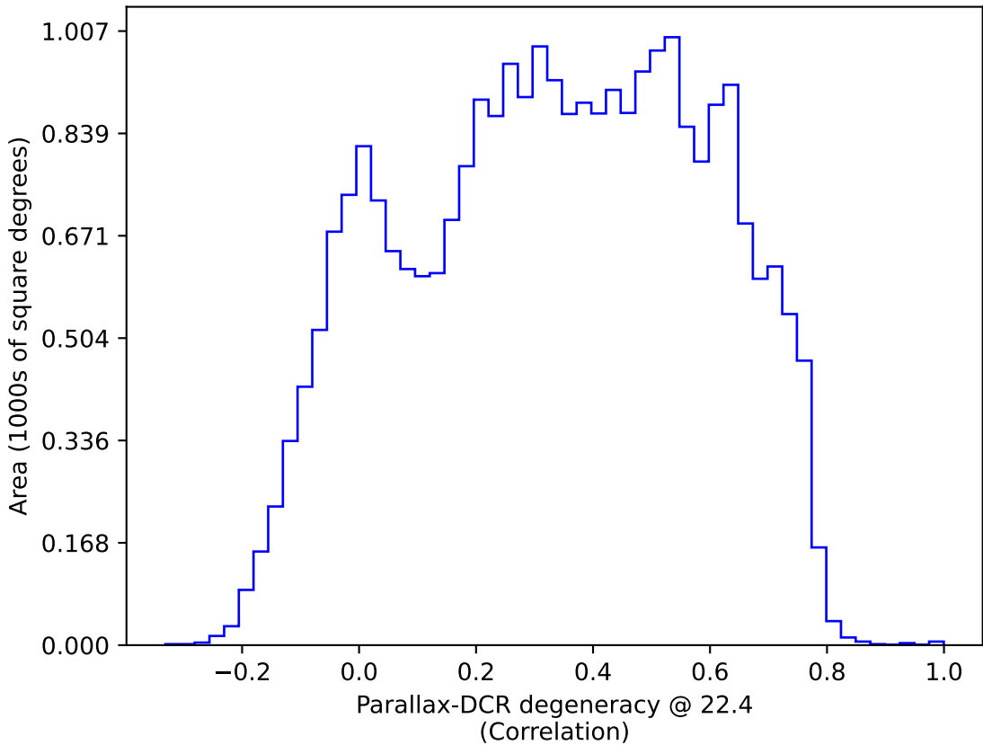
extra_ss_neo3_v3.4_10yrs All sky: Parallax-DCR degeneracy @ 22.4
