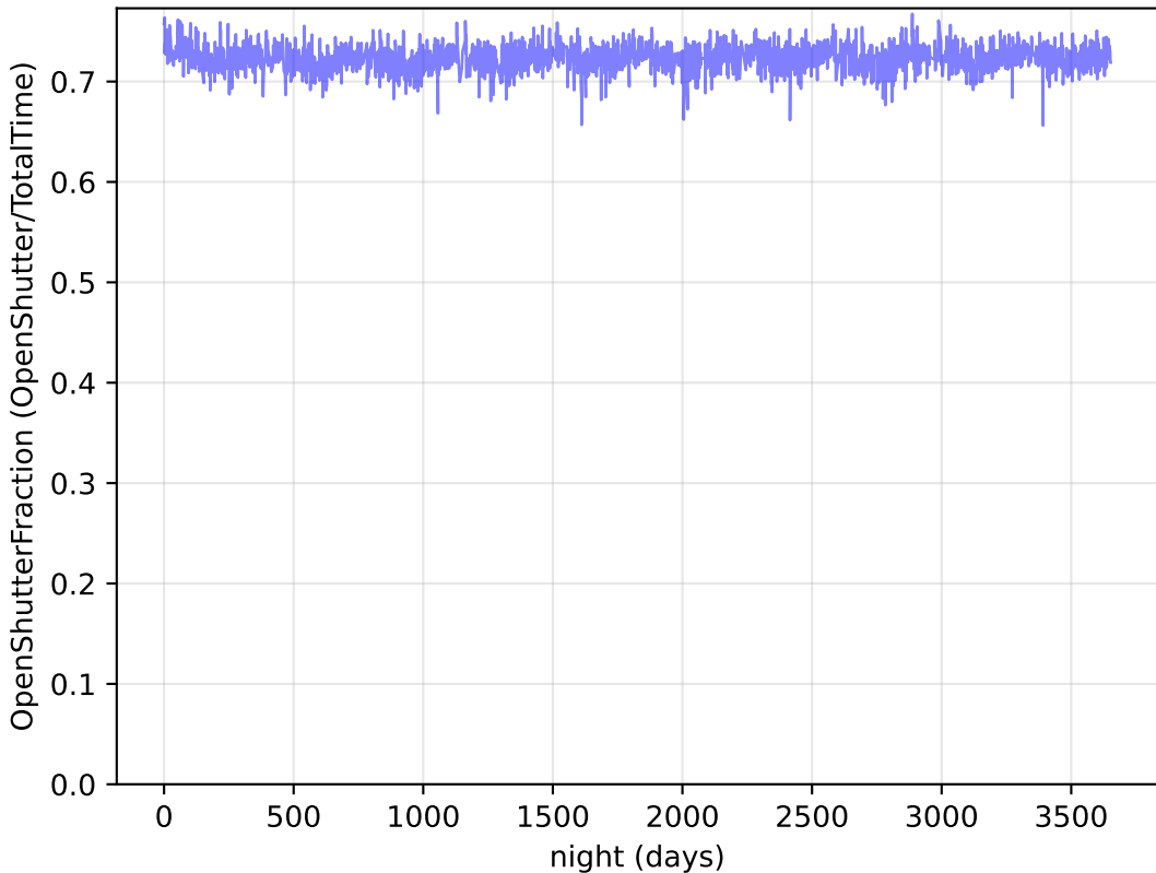
extra_ss_neo3_v3.4_10yrs Per night: OpenShutterFraction
