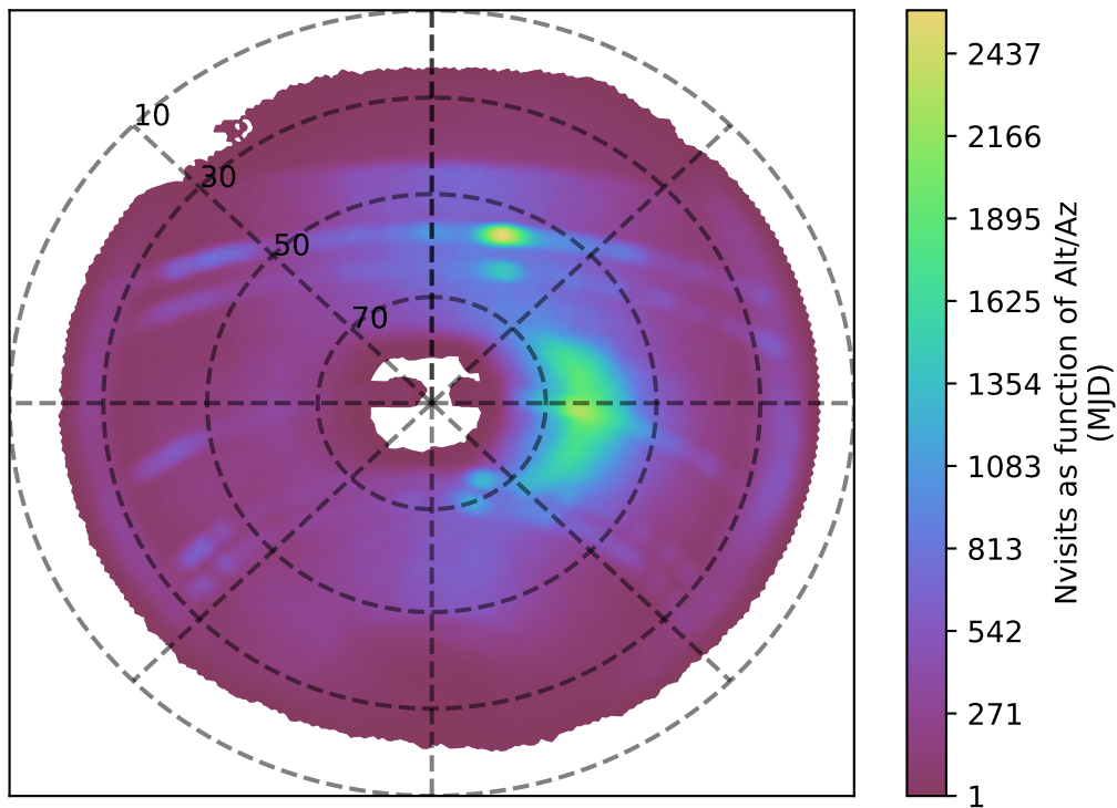
extra_ss_neo3_v3.4_10yrs z band: Nvisits as function of Alt/Az
