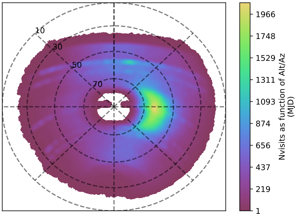
extra_ss_neo3_v3.4_10yrs y band: Nvisits as function of Alt/Az
