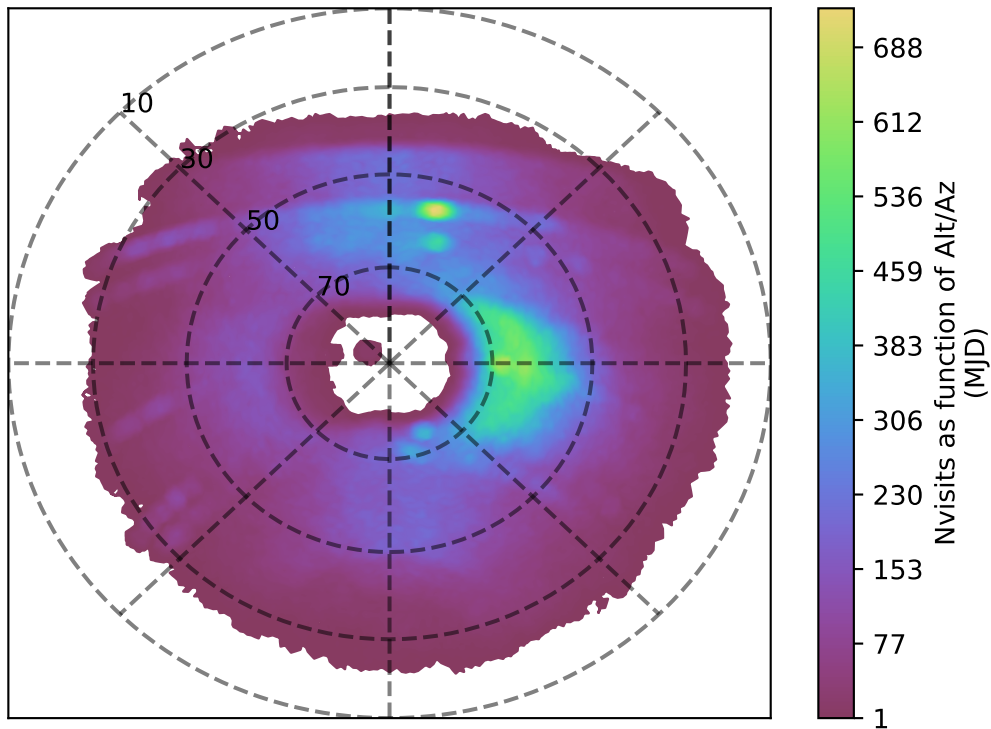
extra_ss_neo3_v3.4_10yrs u band: Nvisits as function of Alt/Az
