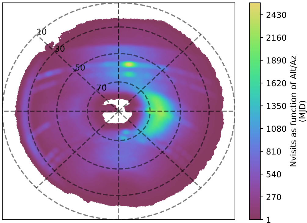
extra_ss_neo3_v3.4_10yrs r band: Nvisits as function of Alt/Az
