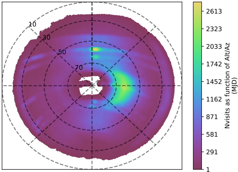
extra_ss_neo3_v3.4_10yrs i band: Nvisits as function of Alt/Az
