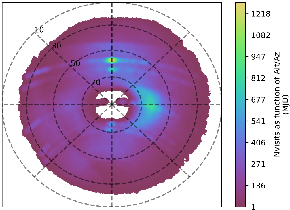
extra_ss_neo3_v3.4_10yrs g band: Nvisits as function of Alt/Az
