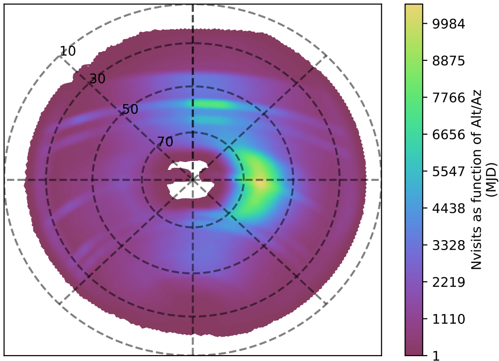
extra_ss_neo3_v3.4_10yrs all bands: Nvisits as function of Alt/Az
