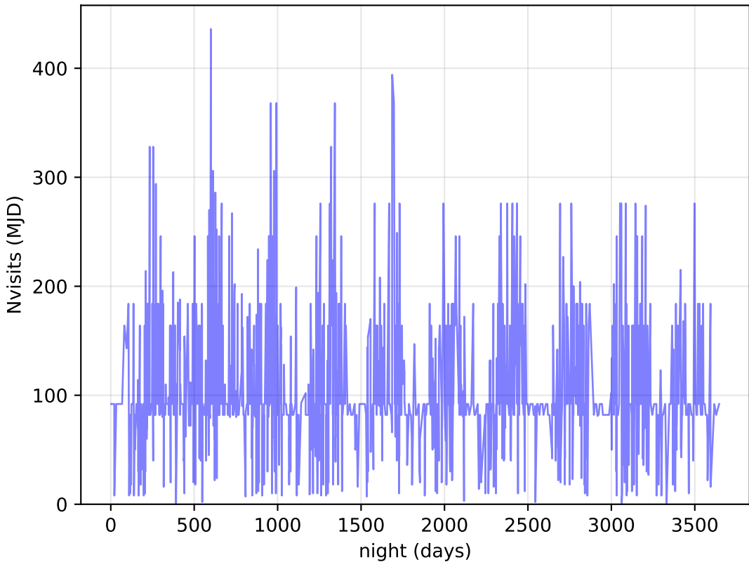
extra_ss_neo3_v3.4_10yrs DDF: Nvisits
