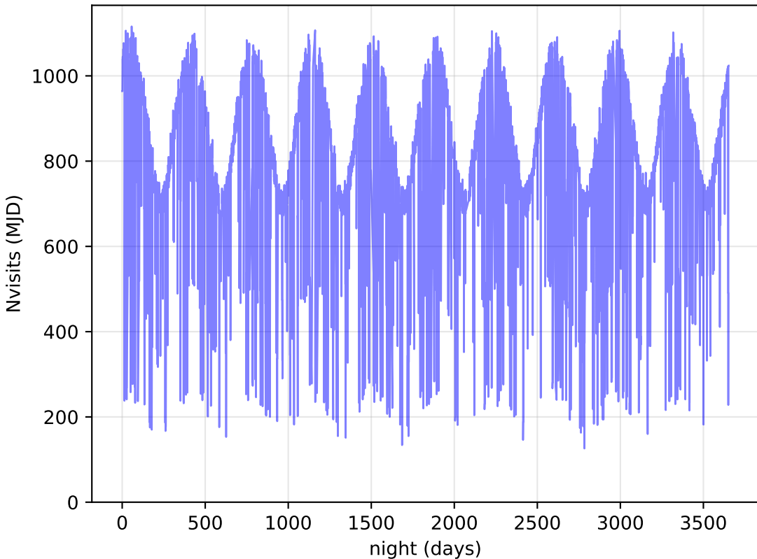
extra_ss_neo3_v3.4_10yrs All visits: Nvisits
