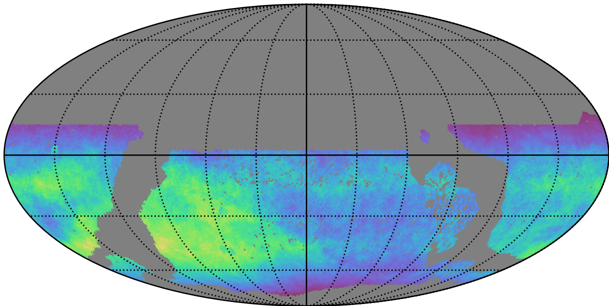
extra_ss_neo3_v3.4_10yrs WFD z band: Normalized Teff
