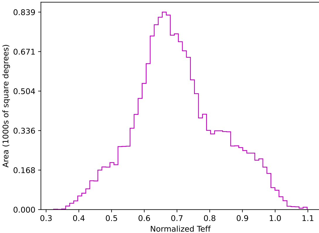
extra_ss_neo3_v3.4_10yrs WFD z band: Normalized Teff
