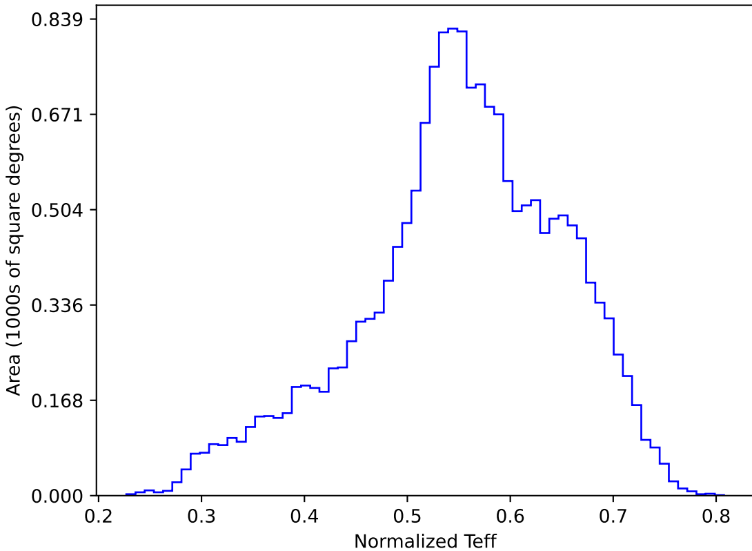
extra_ss_neo3_v3.4_10yrs WFD y band: Normalized Teff
