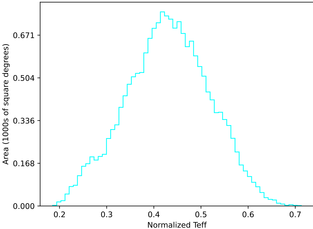
extra_ss_neo3_v3.4_10yrs WFD u band: Normalized Teff
