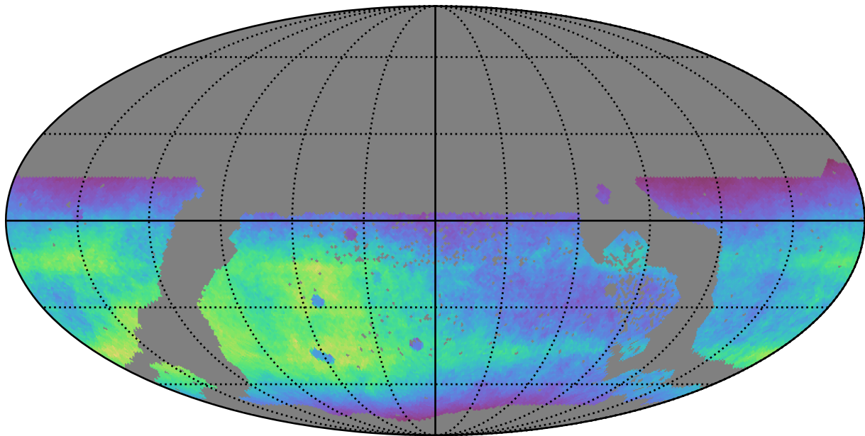
extra_ss_neo3_v3.4_10yrs WFD r band: Normalized Teff
