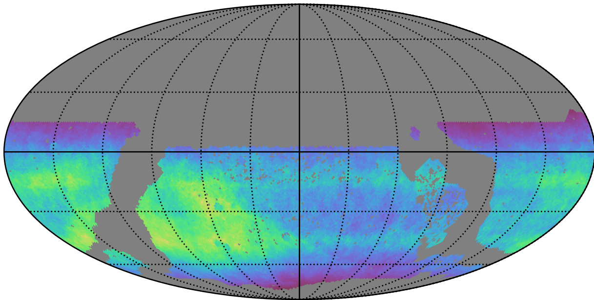
extra_ss_neo3_v3.4_10yrs WFD i band: Normalized Teff
