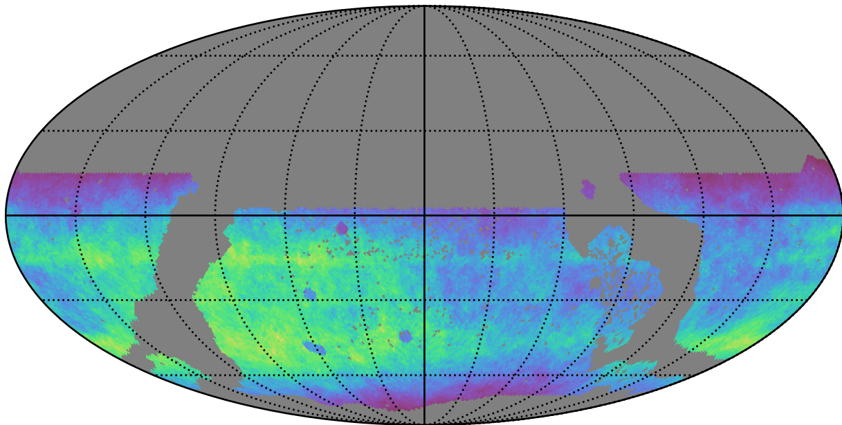
extra_ss_neo3_v3.4_10yrs WFD g band: Normalized Teff
