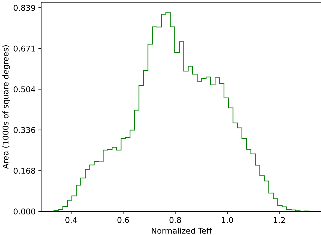
extra_ss_neo3_v3.4_10yrs WFD g band: Normalized Teff
