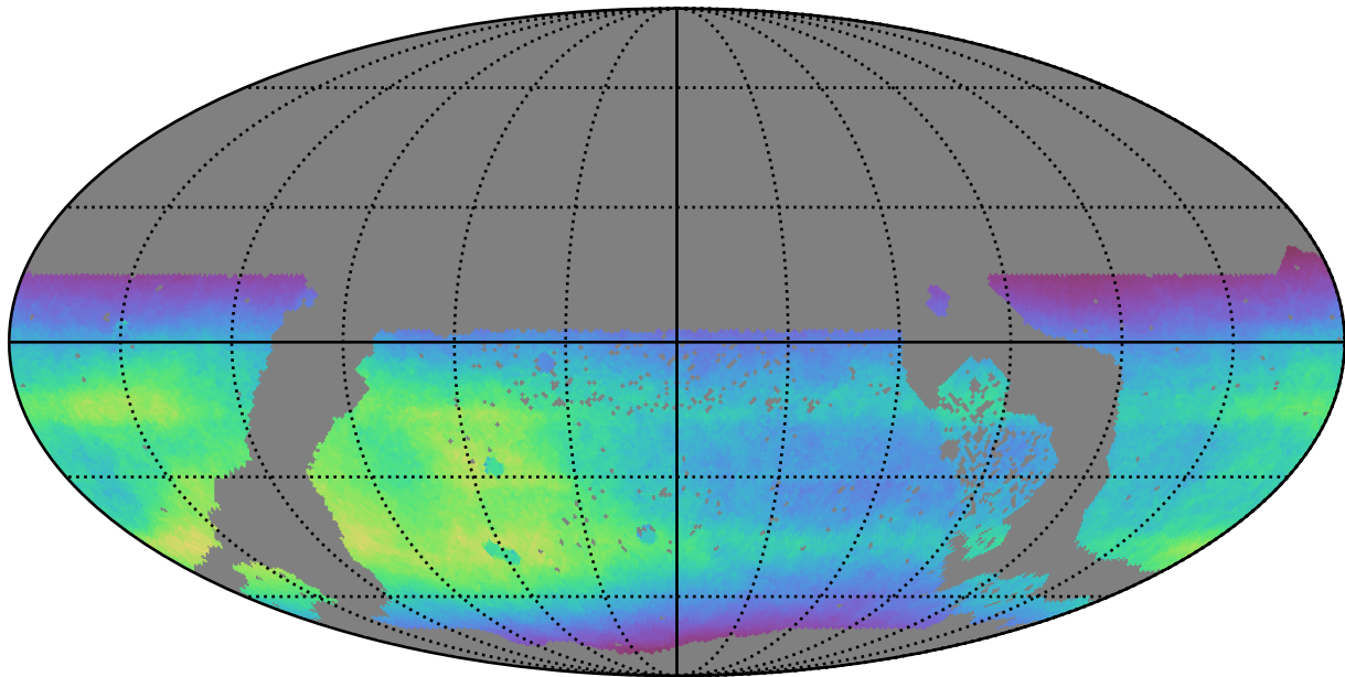
extra_ss_neo3_v3.4_10yrs WFD all bands: Normalized Teff
