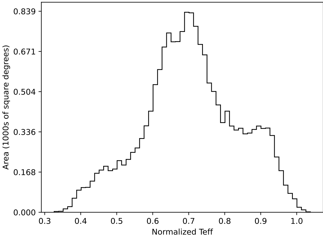
extra_ss_neo3_v3.4_10yrs WFD all bands: Normalized Teff
