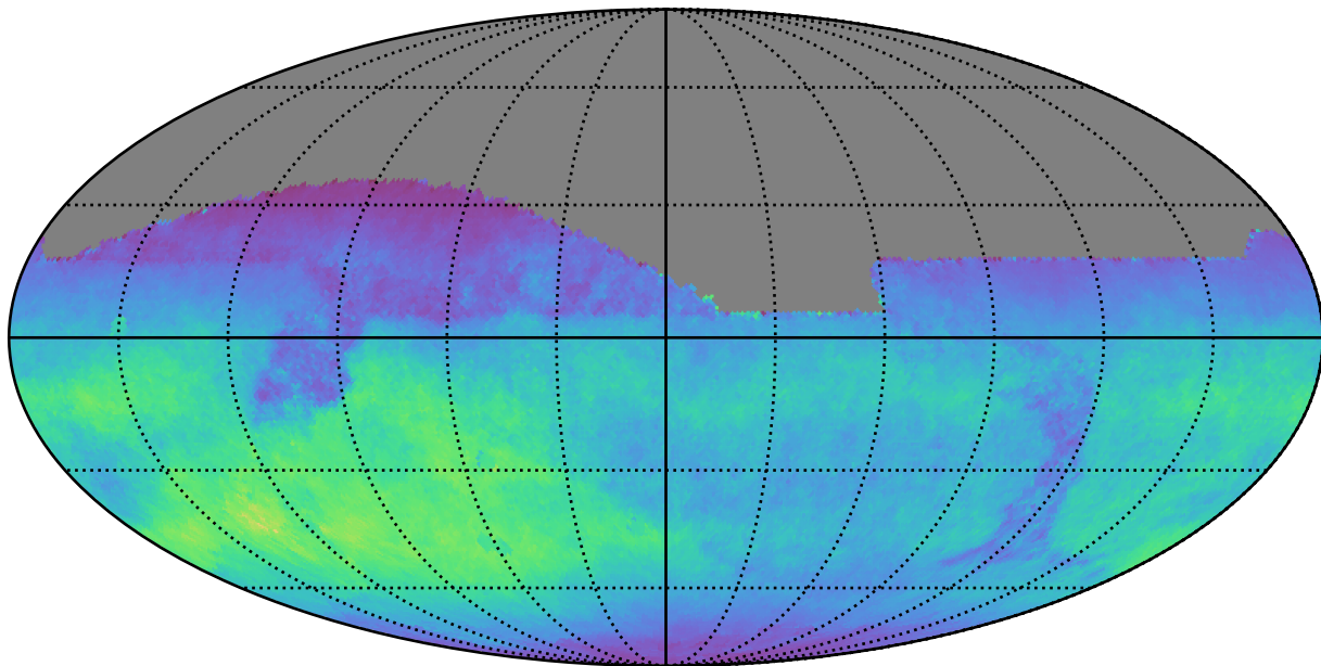
extra_ss_neo3_v3.4_10yrs All sky z band: Normalized Teff
