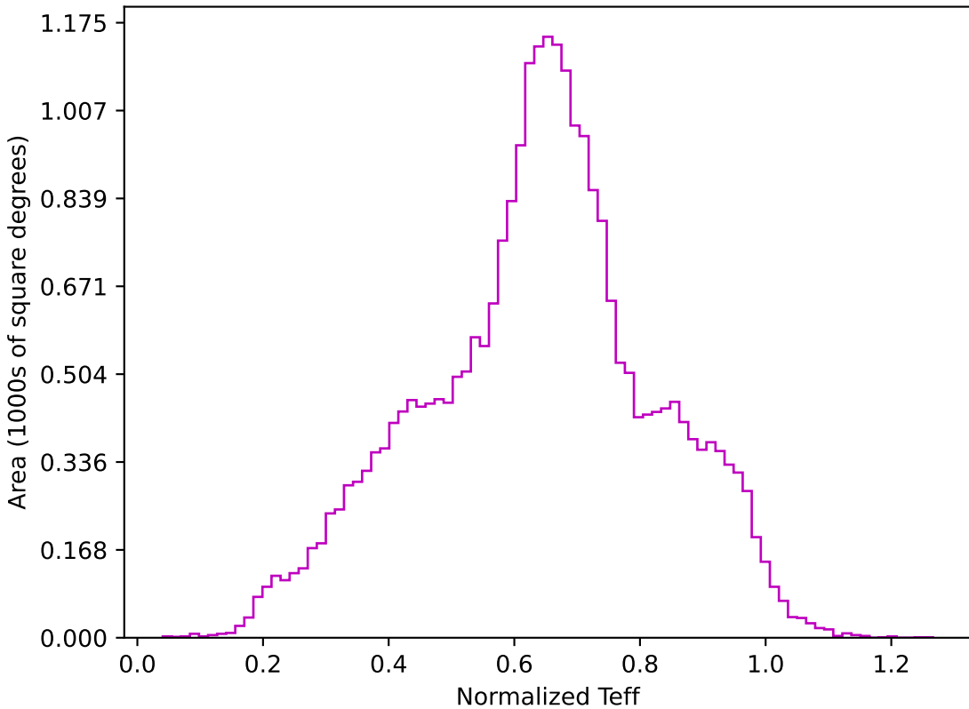
extra_ss_neo3_v3.4_10yrs All sky z band: Normalized Teff
