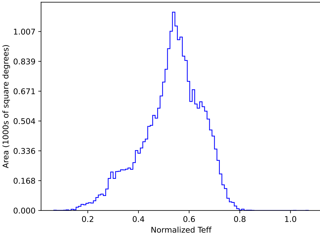
extra_ss_neo3_v3.4_10yrs All sky y band: Normalized Teff
